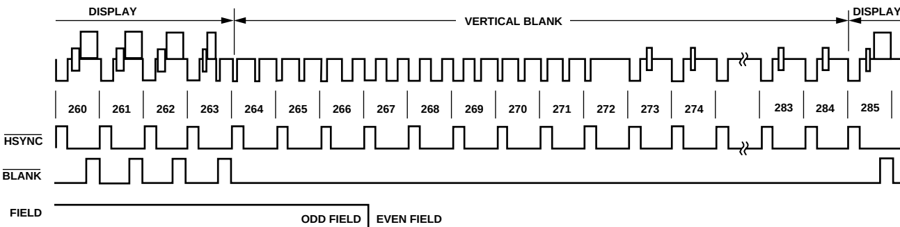
Figure 31. Timing Mode 3 (NTSC)
