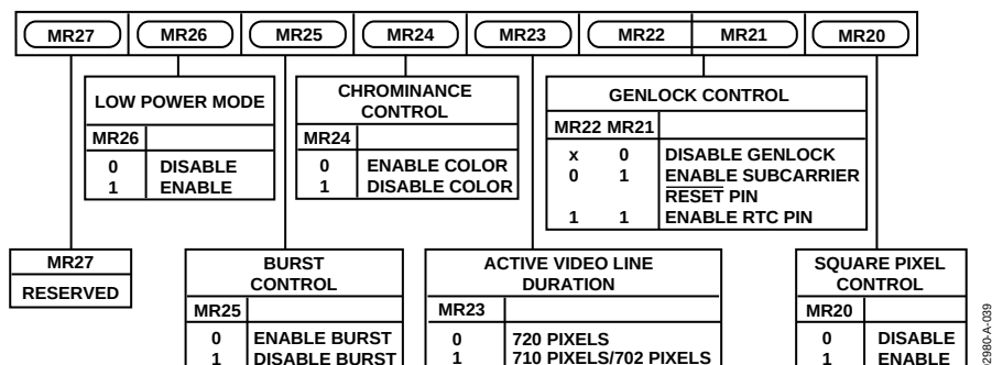
Figure 40. Mode Register 2
