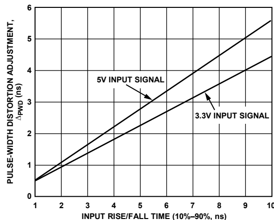
Figure 17. Typical Pulse-Width Distortion Adjustment Due to Input Rise/Fall Time Variation (for V_{DD1} = 3.3\text{ V} and 5\text{ V} )
