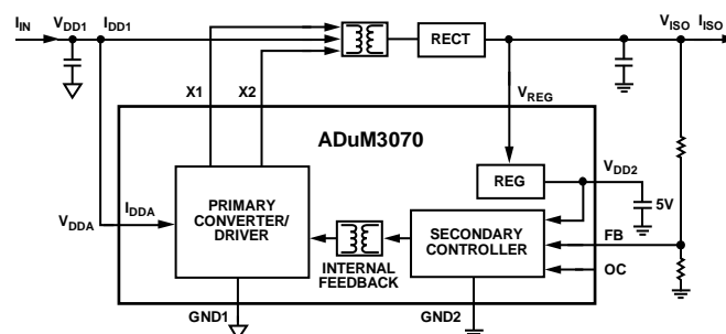
Figure 35. Supply Currents
