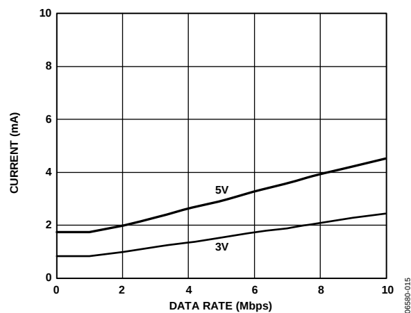
Figure 15. Typical ADuM1412 V_{DD1} or V_{DD2} Supply Current vs. Data Rate for 5 V and 3 V Operation
