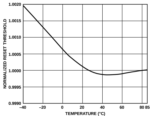
Figure 9. Normalized Reset Voltage Threshold vs. Temperature
