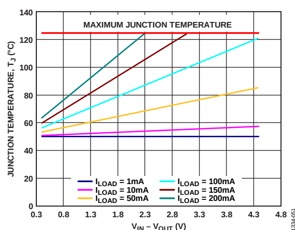
Figure 53. LFCSP, 100 mm 2 of PCB Copper, T_A = 50^\circ\text{C}
