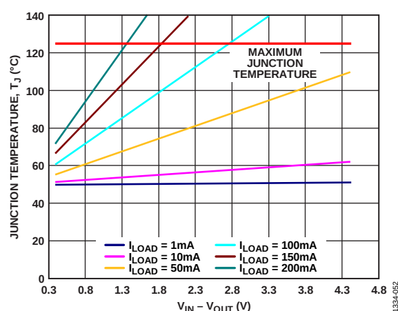
Figure 54. LFCSP, 50 mm 2 of PCB Copper, T_A = 50^\circ\text{C}
