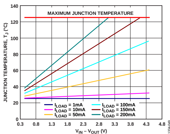
Figure 51. LFCSP, 50 mm 2 of PCB Copper, T_A = 25^\circ\text{C}
