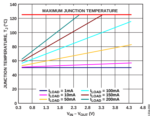
Figure 52. LFCSP, 500 mm 2 of PCB Copper, T_A = 50^\circ\text{C}
