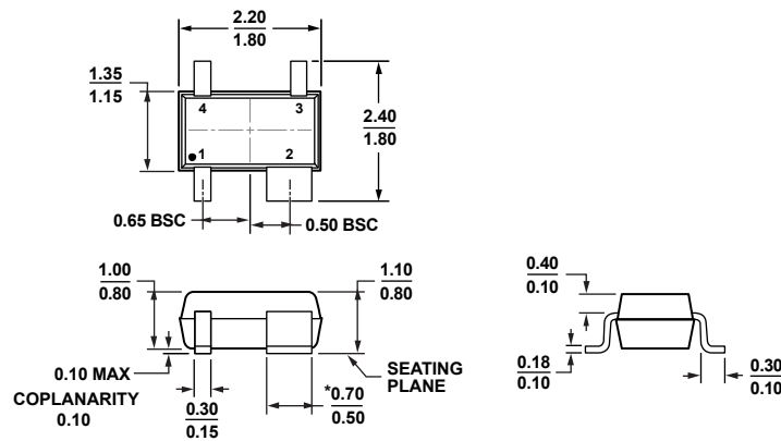
Figure 11. 4-Lead Thin Shrink Small Outline Transistor Package [SC70] (KS-4)
