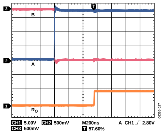
Figure 14. ADM487E Receiver t_{\text{RPHL}}
