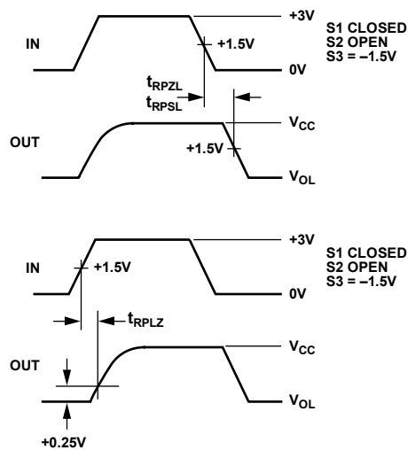
Figure 15. Receiver Enable and Disable Times
