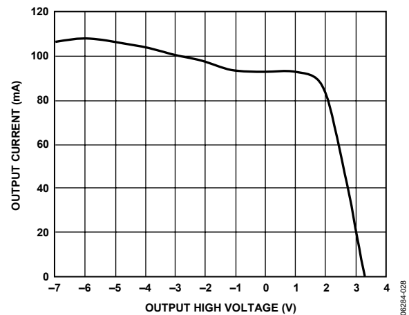
Figure 23. Output Current vs. Driver Output High Voltage
