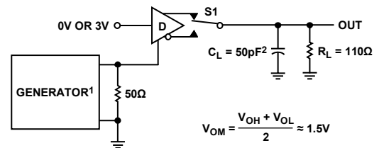
Figure 11. Driver Propagation Delays
