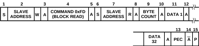
Figure 36. Block Read from EEPROM or RAM with PEC
