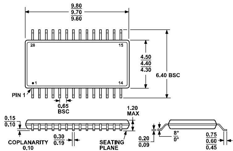
Figure 39. 28-Lead Thin Shrink Small Outline Package [TSSOP] (RU-28)
