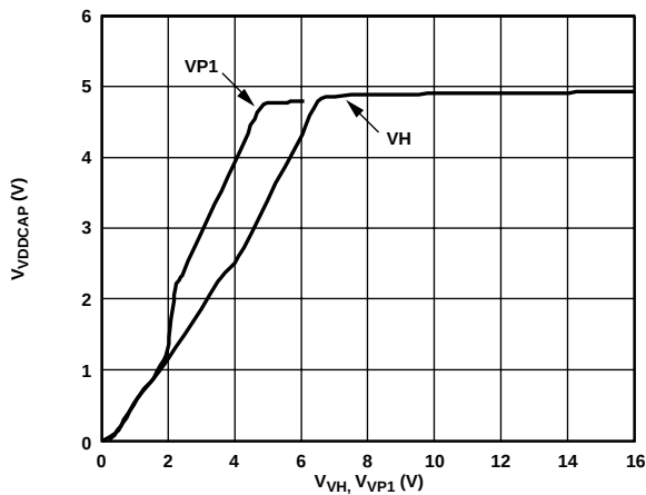
Figure 2. V DDCAP vs. V VH and V VP1
