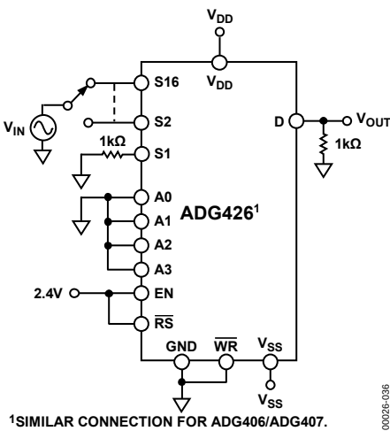
Figure 36. Crosstalk
