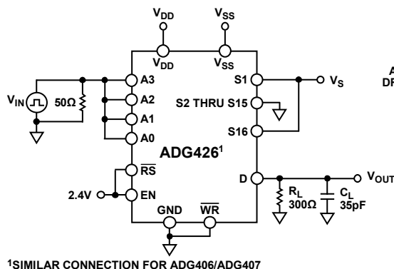
Figure 30. Break-Before-Make Delay, t_{\text{OPEN}}
