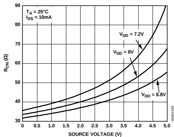
Figure 7. R_{ON} vs. Source Voltage, V_{DD} = 8\text{ V} \pm 10\%
