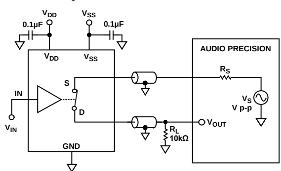
Figure 31. THD + Noise
