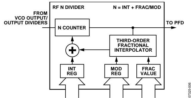
Figure 17. RF INT Divider
