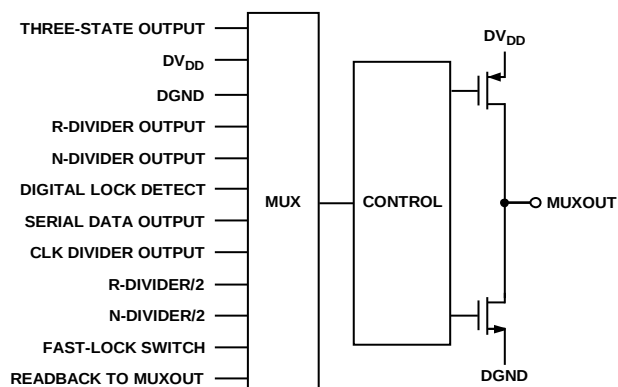
Figure 20. MUXOUT Schematic
