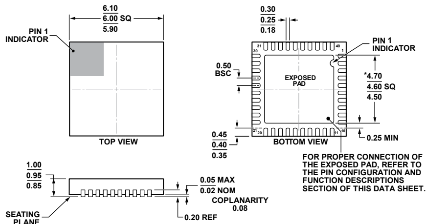
* COMPLIANT TO JEDEC STANDARDS MO-220-VJJD-5 WITH EXCEPTION TO EXPOSED PAD DIMENSION. Figure 51. 40-Lead Lead Frame Chip Scale Package [LFCSP] 6 mm × 6 mm Body and 0.95 mm Package Height (CP-40-15) Dimensions shown in millimeters
