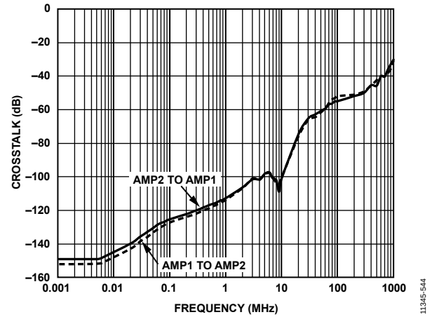
Figure 44. Crosstalk vs. Frequency (MSOP)
