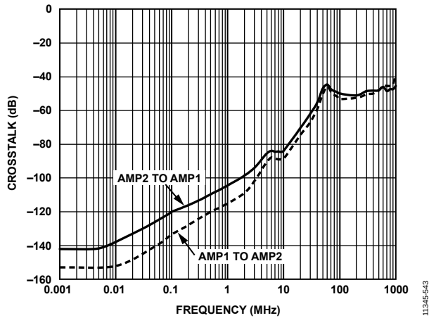
Figure 42. Crosstalk vs. Frequency (LFCSP)
