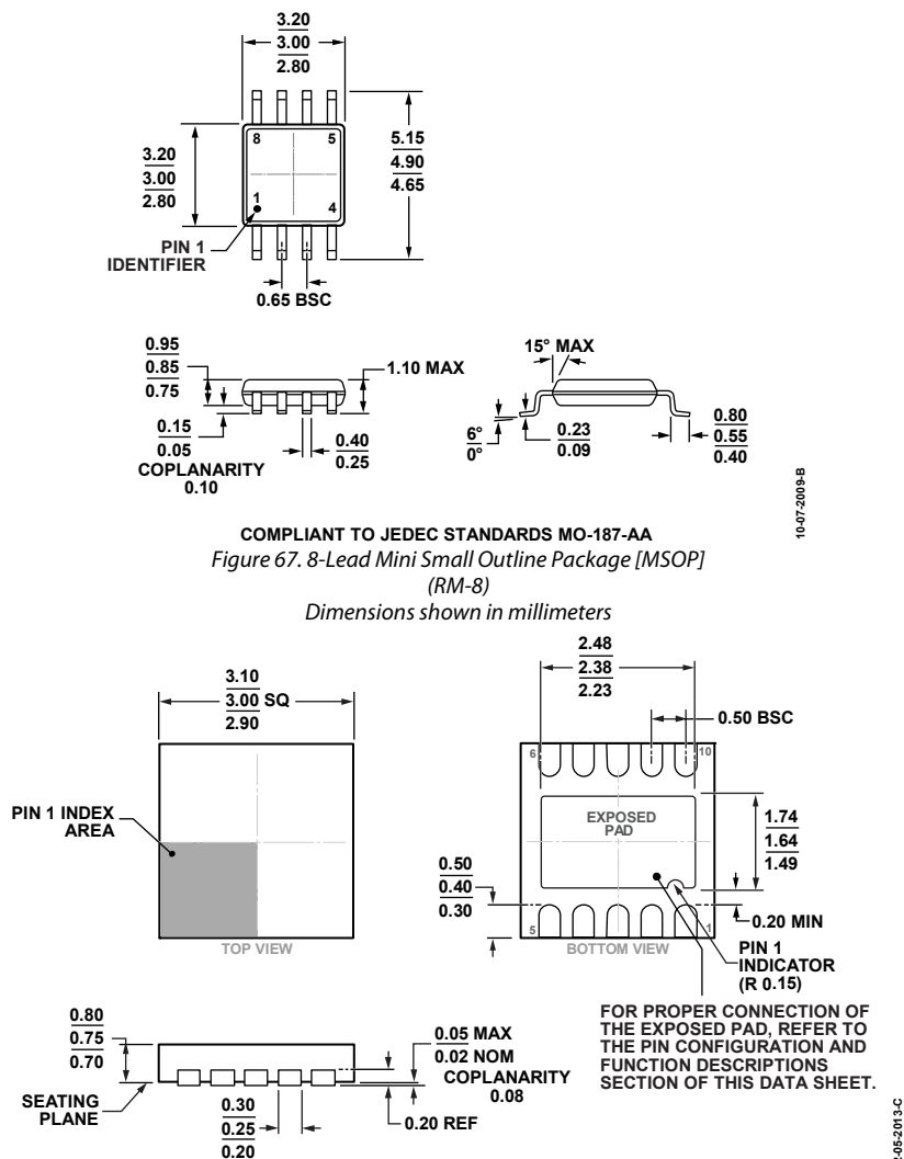
Figure 68. 10-Lead Lead Frame Chip Scale Package [LFCSP_WD] 3 mm × 3 mm Body, Very Very Thin, Dual Lead (CP-10-9)
