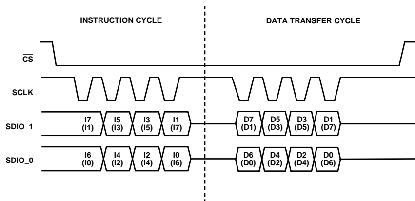
Figure 48. 2-Bit Serial Mode Read Timing—Clock Stall High
