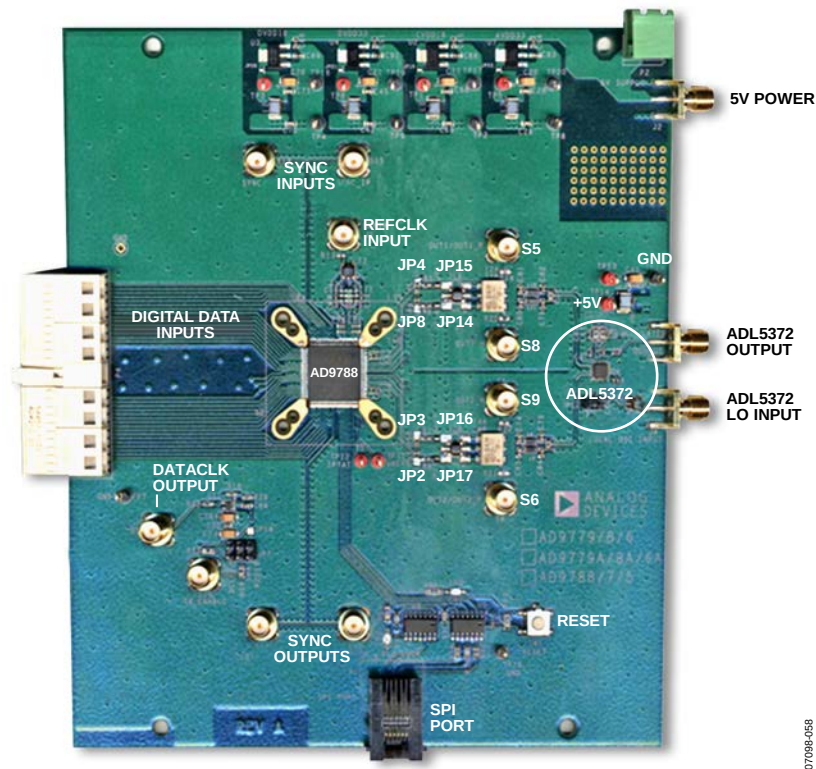
Figure 79. Evaluation Board
