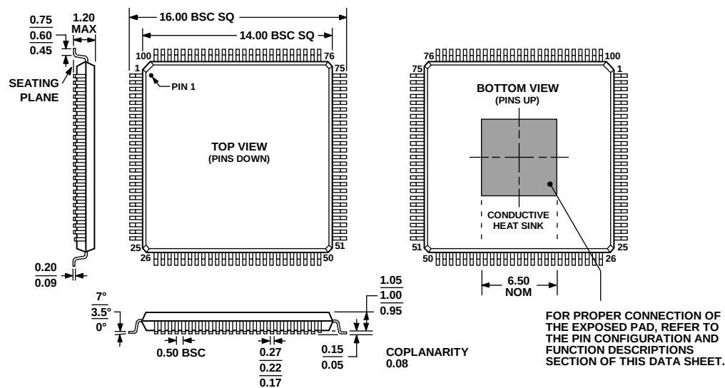
Figure 87. 100-Lead Thin Quad Flat Package, Exposed Pad [TQFP_EP] (SV-100-1) Dimensions shown in millimeters
