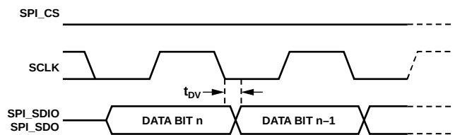
Figure 46. SPI Register Read Timing Instruction Byte
