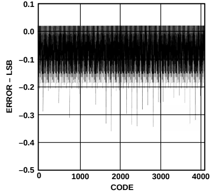
Figure 13. Typical DNL
