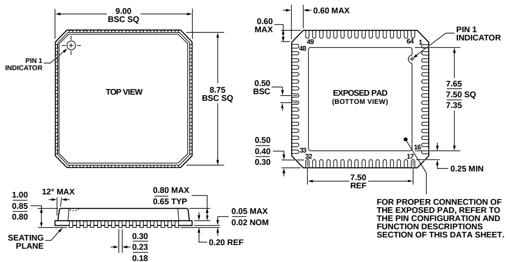
Figure 75. 64-Lead Lead Frame Chip Scale Package [LFCSP_VQ]
