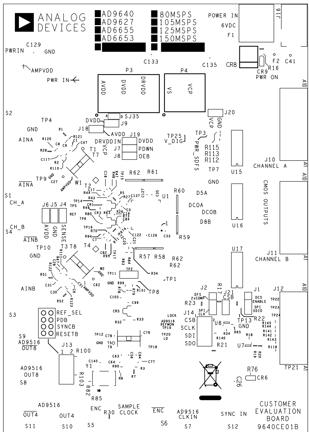
Figure 90. Evaluation Board Layout, Silkscreen, Primary Side
