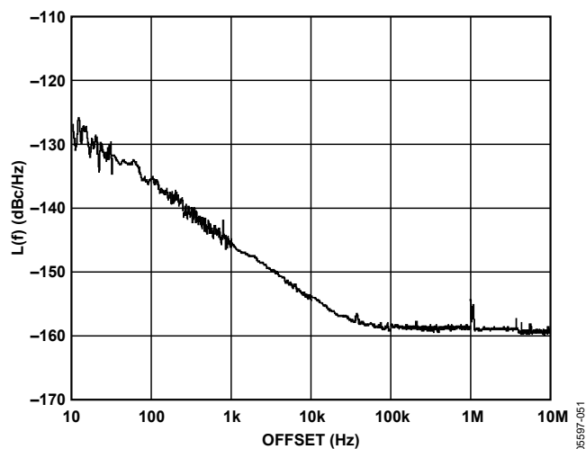
Figure 16. Additive Phase Noise—LVPECL, Divide = 1, 245.76 MHz
