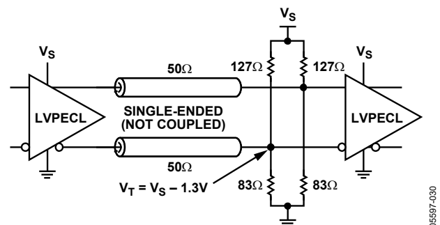
Figure 35. LVPECL Far-End Termination
