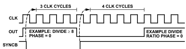
Figure 24. SYNCB Timing with Clock Present
