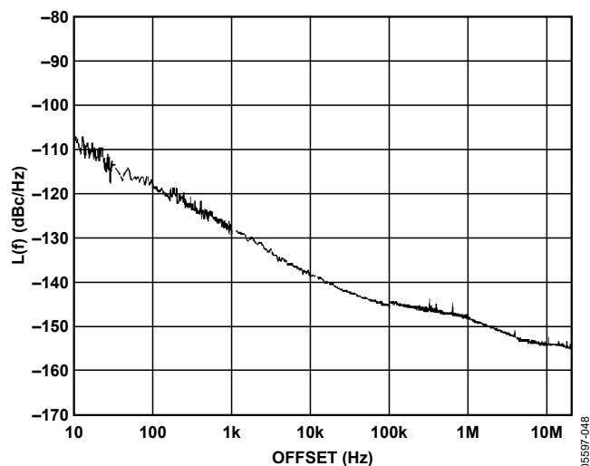
Figure 17. Additive Phase Noise—LVDS, Divide = 1, 245.76 MHz
