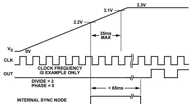
Figure 23. Power-On Sync Timing
