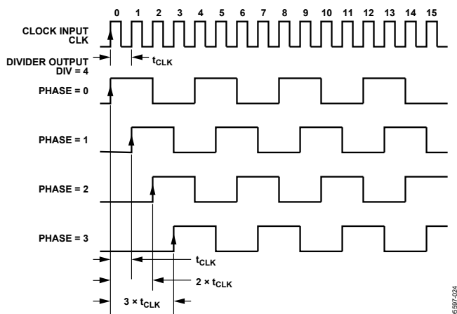
Figure 28. Phase Offset—Divider Set for Divide = 4, Phase Set from 0 to 2
