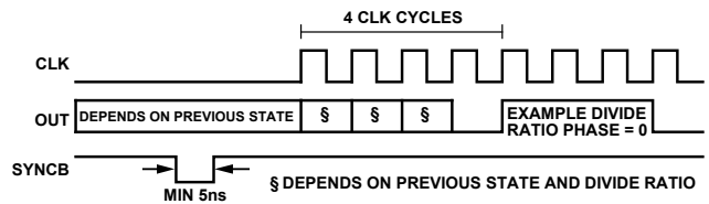
Figure 25. SYNCB Timing with No Clock Present
