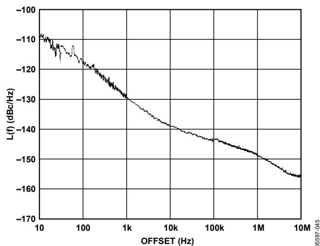
Figure 18. Additive Phase Noise—CMOS, Divide = 1, 245.76 MHz
