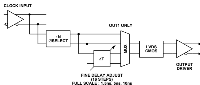
Figure 29. Analog Delay Block
