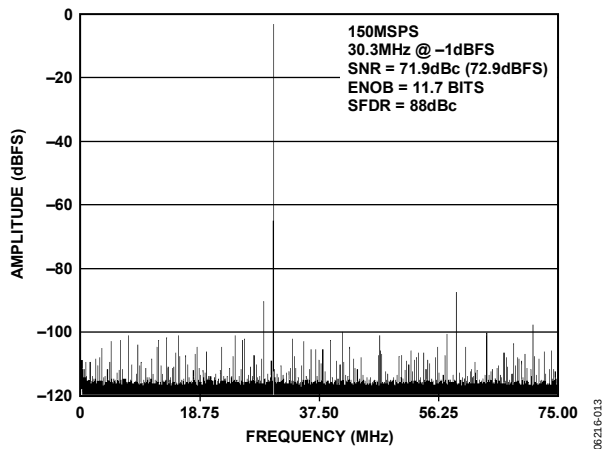
Figure 13. AD9254 Single-Tone FFT with f_{IN} = 30.3 MHz
