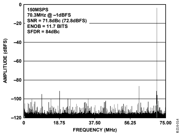
Figure 14. AD9254 Single-Tone FFT with f_{IN} = 70.3 MHz
