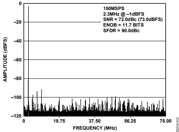
Figure 12. AD9254 Single-Tone FFT with f_{IN} = 2.3 MHz
