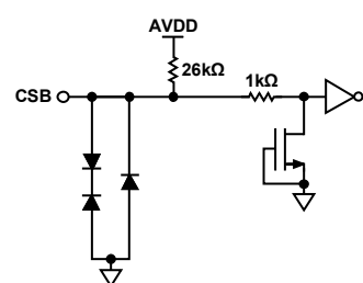
Figure 9. Equivalent CSB Input Circuit
