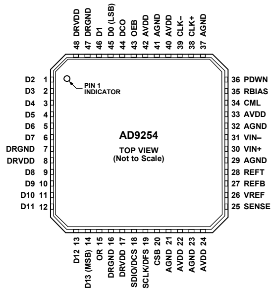
Figure 3. Pin Configuration
