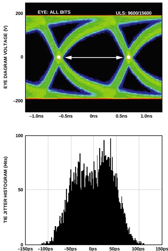
Figure 51. Data Eye for LVDS Outputs in ANSI-644 Mode with Trace Lengths Greater than 24 Inches on Standard FR-4, External 100 Ω Far Termination Only
