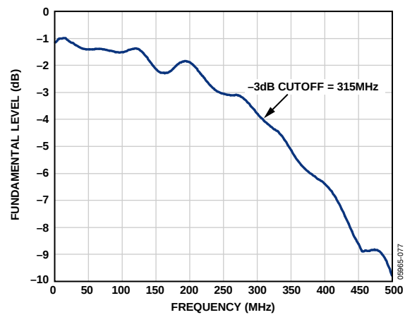
Figure 34. Full-Power Bandwidth vs. Frequency, f_{\text{SAMPLE}} = 50 \text{ MSPS}
