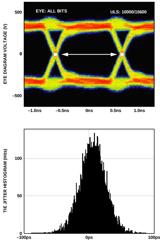
Figure 50. Data Eye for LVDS Outputs in ANSI-644 Mode with Trace Lengths Less than 24 Inches on Standard FR-4, External 100 Ω Far Termination Only
