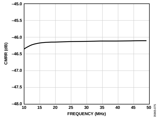
Figure 31. CMRR vs. Frequency, f_{\text{SAMPLE}} = 50 \text{ MSPS}
