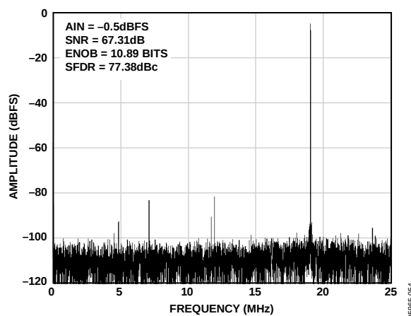
Figure 18. Single-Tone 32k FFT with f_{IN} = 170 MHz, f_{SAMPLE} = 50 MSPS
