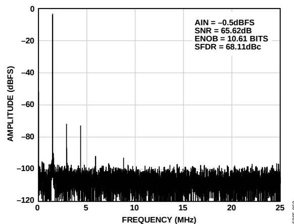
Figure 20. Single-Tone 32k FFT with f_{IN} = 250 MHz, f_{SAMPLE} = 50 MSPS
