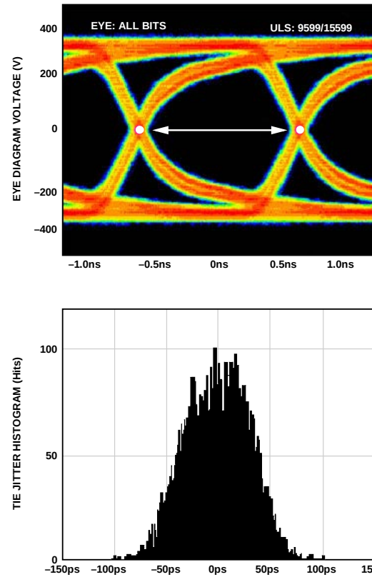
Figure 52. Data Eye for LVDS Outputs in ANSI-644 Mode with 100 Ω Internal Termination on and Trace Lengths Greater than 24 Inches on Standard FR-4, External 100 Ω Far Termination Only
