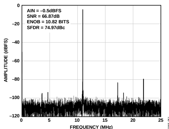
Figure 19. Single-Tone 32k FFT with f_{IN} = 190 MHz, f_{SAMPLE} = 50 MSPS
