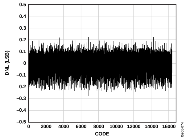
Figure 30. DNL, f_{\text{IN}} = 2.4 \text{ MHz} , f_{\text{SAMPLE}} = 50 \text{ MSPS}
