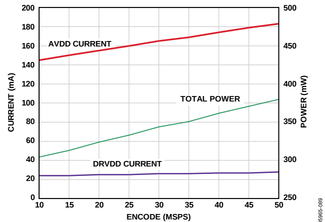
Figure 48. Supply Current vs. f_{\text{SAMPLE}} for f_{\text{IN}} = 10.3 \text{ MHz} , f_{\text{SAMPLE}} = 50 \text{ MSPS}
