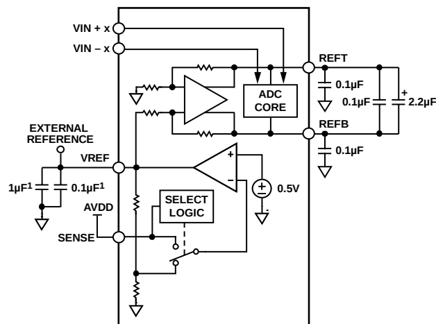
Figure 54. External Reference Operation
