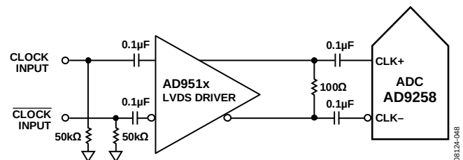
Figure 78. Differential LVDS Sample Clock (Up to 625 MHz)
