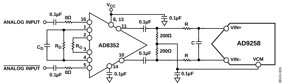
Figure 69. Differential Input Configuration Using the AD8352
