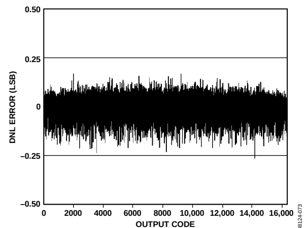
Figure 19. AD9258-80 DNL with f_{IN} = 9.7 MHz
