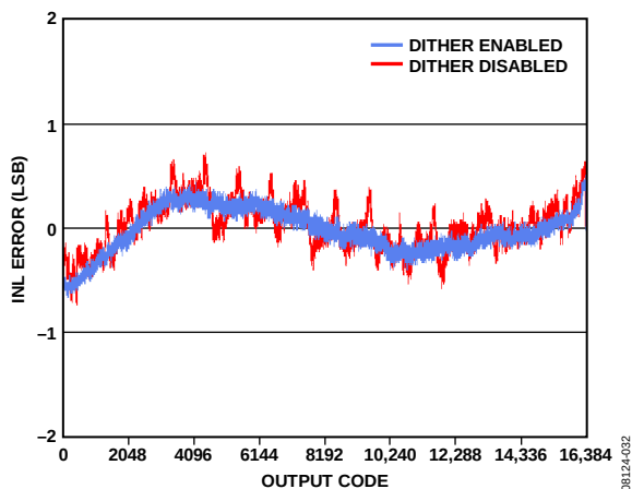
Figure 52. AD9258-125 INL with f_{IN} = 9.7 MHz
