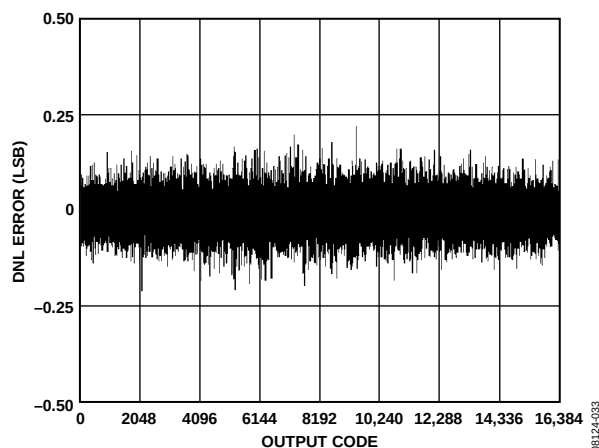
Figure 53. AD9258-125 DNL with f_{IN} = 9.7 MHz
