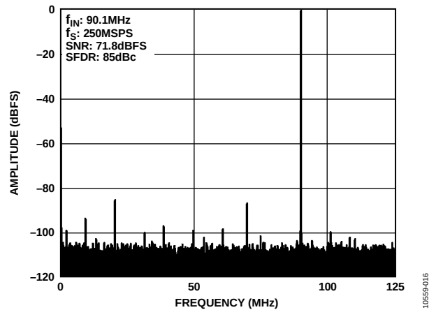
Figure 16. AD9250-250 Single-Tone FFT with f_{IN} = 90.1 MHz
