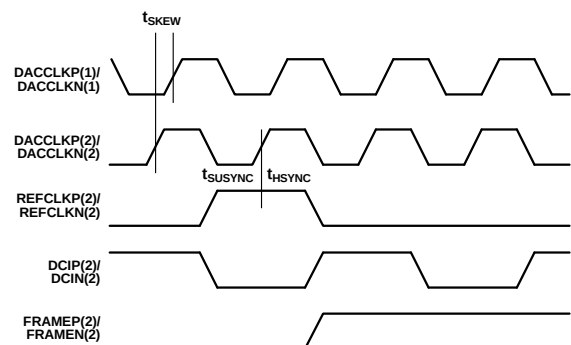
Figure 85. FIFO Rate Synchronization Signal Timing Requirements, 2x Interpolation
