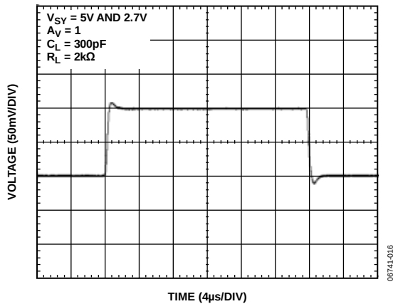
Figure 19. AD8538 Small Signal Transient Response
