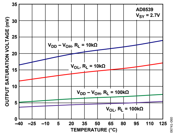
Figure 59. AD8539 Output Saturation Voltage vs. Temperature
