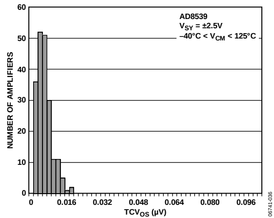
Figure 35. AD8539 Input Offset Voltage Drift Distribution
