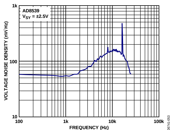
Figure 52. AD8539 Voltage Noise Density
