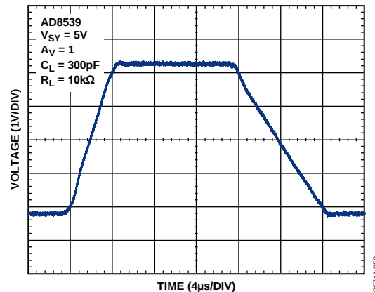
Figure 49. AD8539 Large Signal Transient Response
