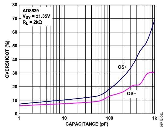
Figure 60. AD8539 Small Signal Overshoot vs. Load Capacitance
