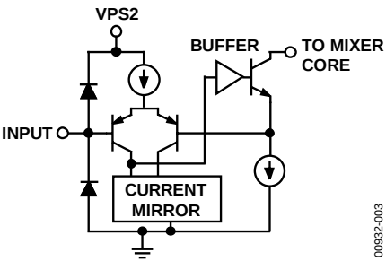
Figure 23. Circuit A
