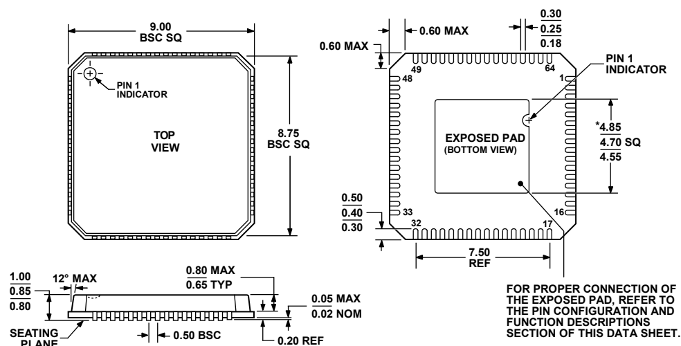
Figure 69. 64-Lead Lead Frame Chip Scale Package [LFCSP_VQ] 9 mm × 9 mm Body, Very Thin Quad (CP-64-1)
