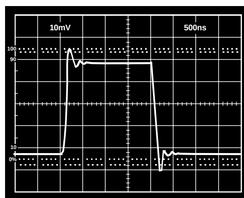
Figure 33. Small Signal Response Unity-Gain Follower; V_S = \pm 15 V, R_L = 10 kΩ
