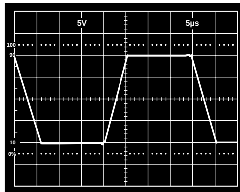
Figure 32. Large Signal Response Unity-Gain Follower; V_S = \pm 15 V, R_L = 10 kΩ
