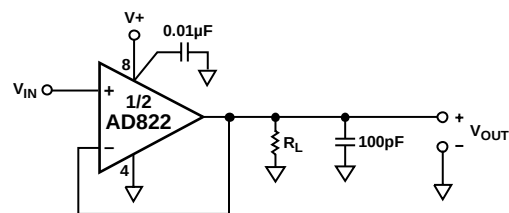
Figure 35. Unity-Gain Follower
