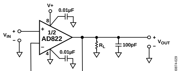
Figure 29. Unity-Gain Follower
