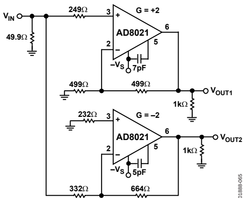
Figure 65. Differential Amplifier
