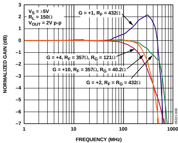
Figure 7. Large Signal Frequency Response vs. Various Gains
