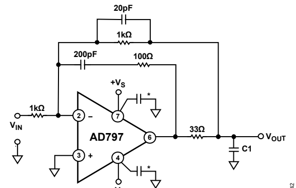
*USE THE POWER SUPPLY BYPASSING SHOWN IN FIGURE 35. Figure 43. Recommended Circuit for Driving a High Capacitance Load
