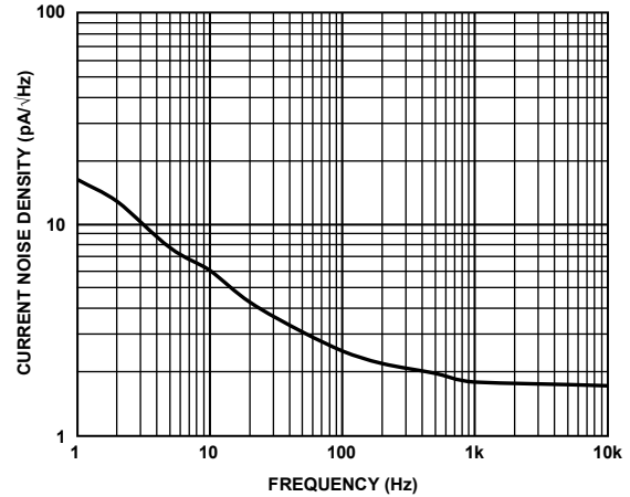
Figure 18. Current Noise Density V_S = \pm 15\text{ V}
