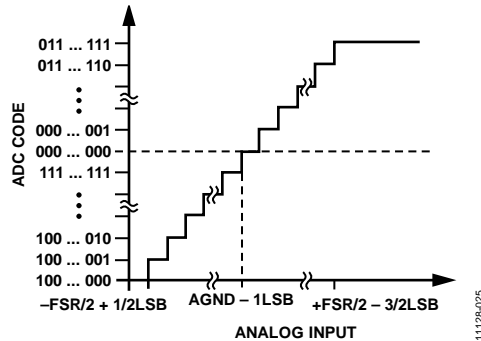
Figure 22. Transfer Characteristic
