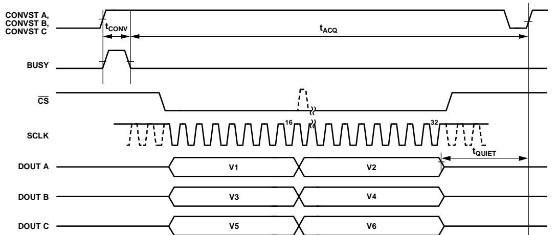
Figure 28. Serial Interface with Three DOUT x Lines
