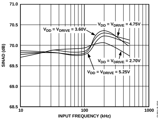
Figure 9. AD7495 SINAD vs. Input Frequency at 1 MSPS
