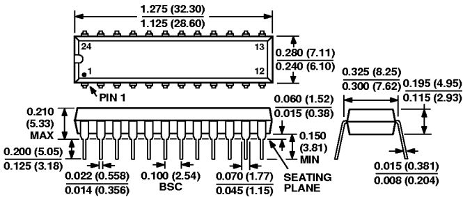
24-Lead Narrow Body Plastic DIP Package (N-24)
