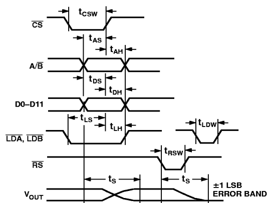
Figure 2. Timing Diagram
