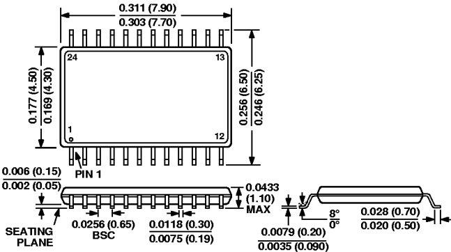
24-Lead Thin Surface Mount TSSOP Package (RU-24)
