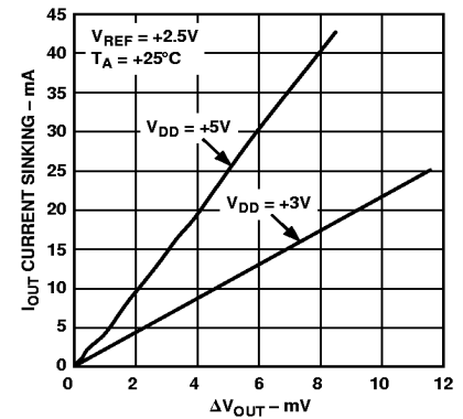
Figure 18. I_{OUT} Sink Current vs. \Delta V_{OUT}
