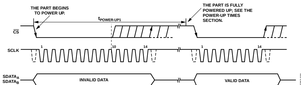
Figure 27. Exiting Partial Power-Down Mode
