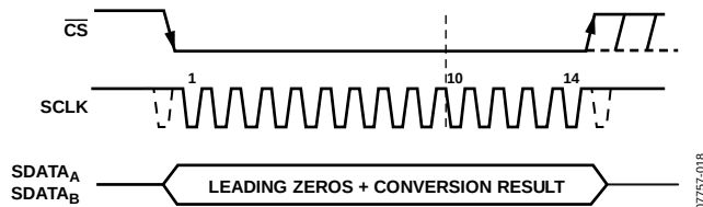
Figure 25. Normal Mode Operation
