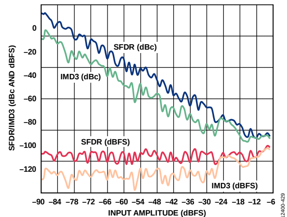
Figure 40. Two-Tone SFDR/IMD3 vs. Input Amplitude ( A_{IN} ) with f_{IN1} = 338\text{ MHz} and f_{IN2} = 341\text{ MHz}
