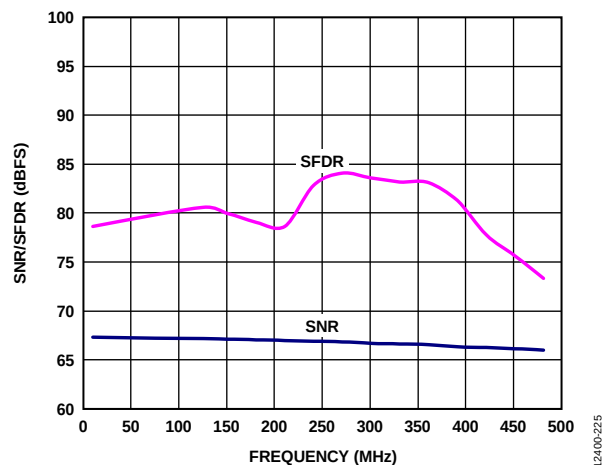
Figure 36. SNR/SFDR vs. Analog Input Frequency ( f_{IN} ); f_{IN} < 500\text{ MHz} ; Buffer Control 1 = 3.0x
