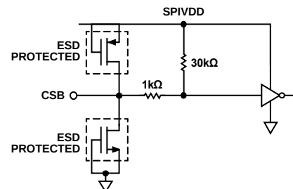
Figure 68. SCLK Inputs
