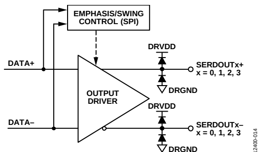
Figure 66. Digital Outputs
