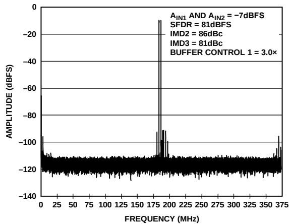
Figure 37. Two-Tone FFT; f_{IN1} = 184\text{ MHz} , f_{IN2} = 187\text{ MHz}
