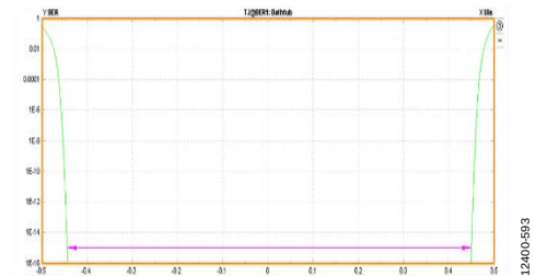
Figure 134. Bathtub, External 100 \Omega Terminations at 7.37 Gbps
