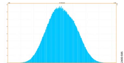
Figure 136. Histogram, External 100 \Omega Terminations at 6 Gbps
