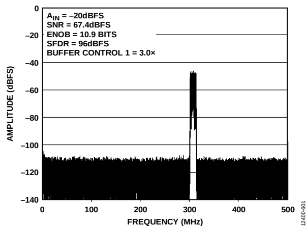
Figure 34. LTE-FDD 10 MHz Channel FFT with f_{IN} = 230\text{ MHz}
