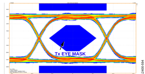
Figure 135. Digital Output Data Eye, External 100 \Omega Terminations at 6 Gbps
