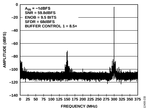
Figure 33. Single Tone FFT with f_{IN} = 1950.3\text{ MHz}
