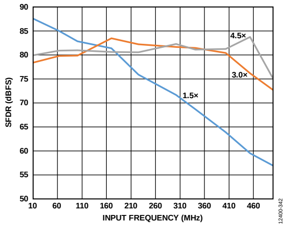
Figure 77. Buffer Current Sweeps, AD6674-1000 (SFDR vs. Input Frequency and I_{BUFF} ); 10 MHz < f_{IN} < 500 MHz; Front-End Network Shown in Figure 74
