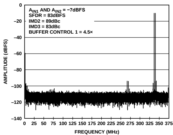
Figure 38. Two-Tone FFT; f_{IN1} = 338\text{ MHz} , f_{IN2} = 341\text{ MHz}
