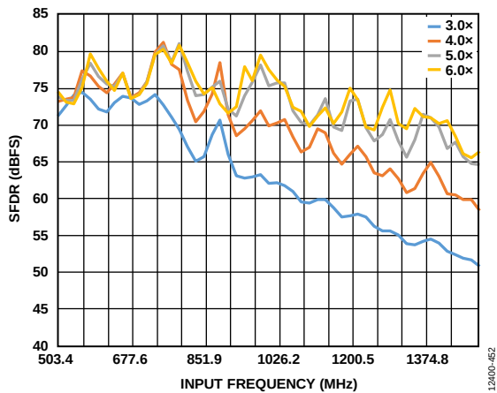
Figure 78. Buffer Current Sweeps, AD6674-1000 (SFDR vs. Input Frequency and I_{BUFF} ); 500 MHz < f_{IN} < 1500 MHz; Front-End Network Shown in Figure 74
