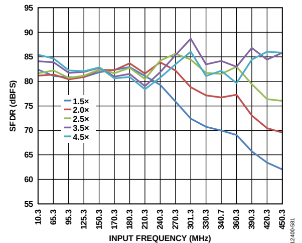
Figure 81. Buffer Current Sweeps, AD6674-750 (SFDR vs. Input Frequency and I_{BUFF} ); 10 MHz < f_{IN} < 450 MHz; Front-End Network Shown in Figure 74
