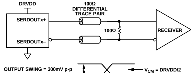
Figure 128. DC-Coupled Digital Output Termination Example
