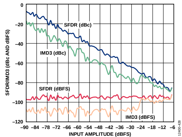
Figure 39. Two-Tone SFDR/IMD3 vs. Input Amplitude ( A_{IN} ) with f_{IN1} = 184\text{ MHz} and f_{IN2} = 187\text{ MHz}
