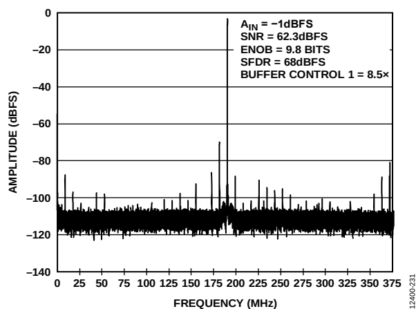
Figure 31. Single Tone FFT with f_{IN} = 1310.3\text{ MHz}
