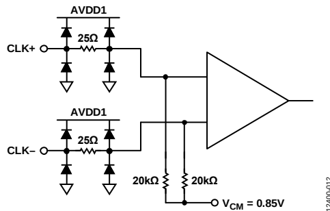
Figure 64. Clock Inputs
