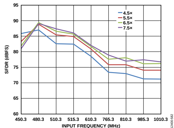
Figure 82. Buffer Current Sweeps, AD6674-750 (SFDR vs. Input Frequency and I_{BUFF} ); 450 MHz < f_{IN} < 800 MHz; Front-End Network Shown in Figure 74
