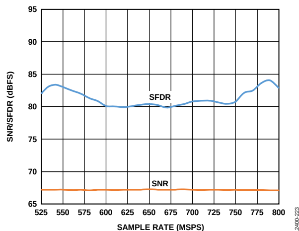
Figure 35. SNR/SFDR vs. Sample Rate ( f_s ); f_{IN} = 170.3\text{ MHz} , Buffer Control 1 = 3.0x
