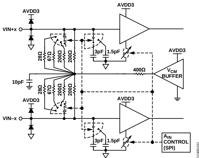
Figure 63. Analog Inputs
