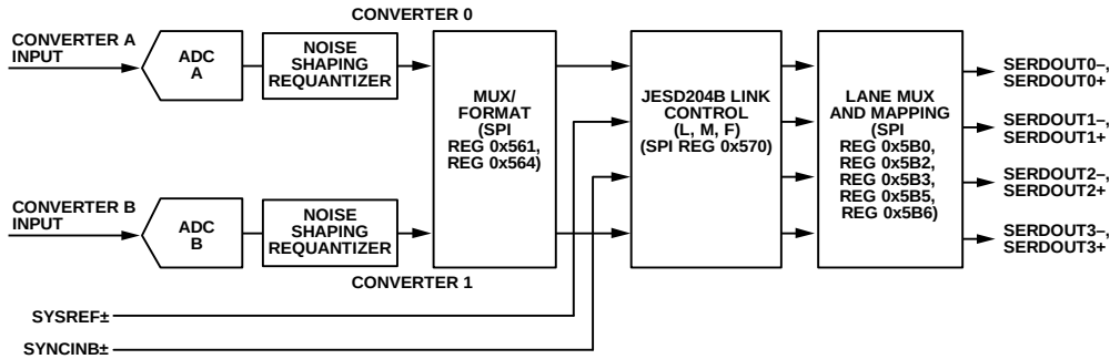
Figure 123. Transmit Link Simplified Block Diagram Showing NSR Mode (Register 0x200 = 0x07)
