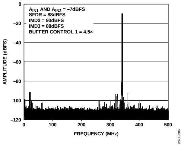
Figure 19. Two-Tone FFT; f_{IN1} = 338 MHz, f_{IN2} = 341 MHz
