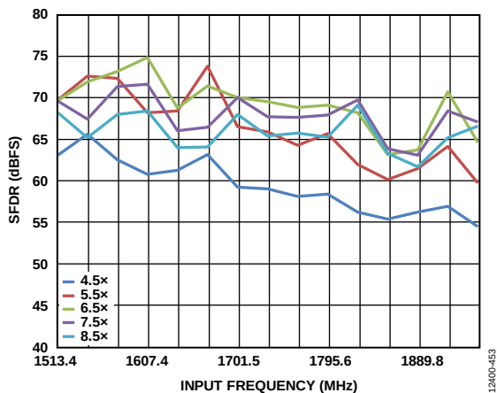
Figure 79. Buffer Current Sweeps, AD6674-1000 (SFDR vs. Input Frequency and I_{BUFF} ); 1500 MHz < f_{IN} < 2 GHz; Front-End Network Shown in Figure 74
