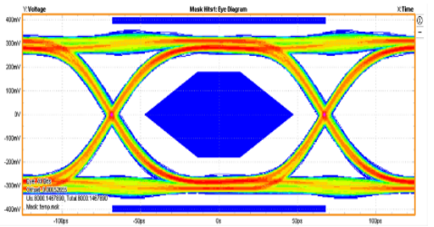
Figure 132. Digital Output Data Eye, External 100 \Omega Terminations at 7.37 Gbps
