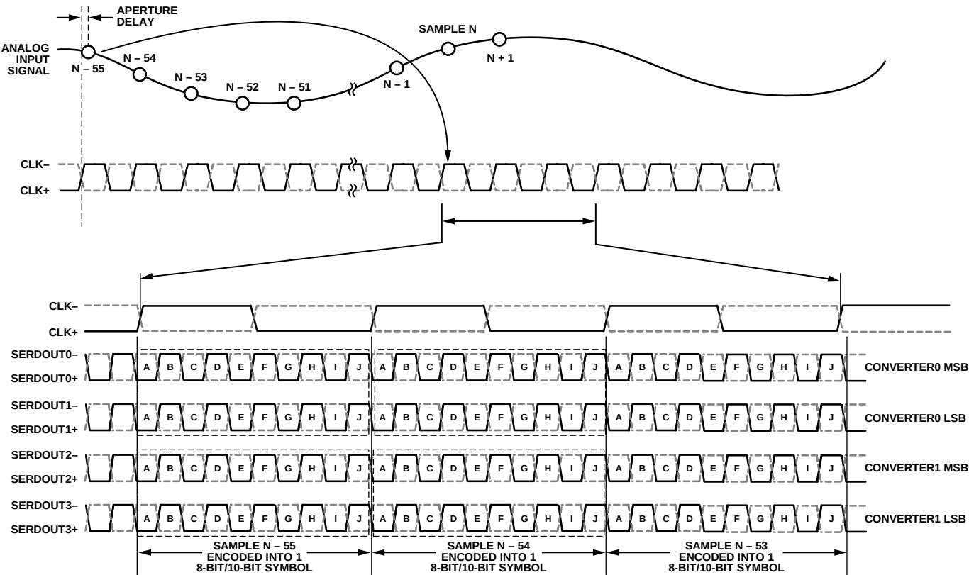
Figure 2. Data Output Timing (VDR Mode; L = 4; M = 2; F = 1)
