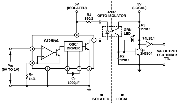
Figure 9. Optoisolator Interface
