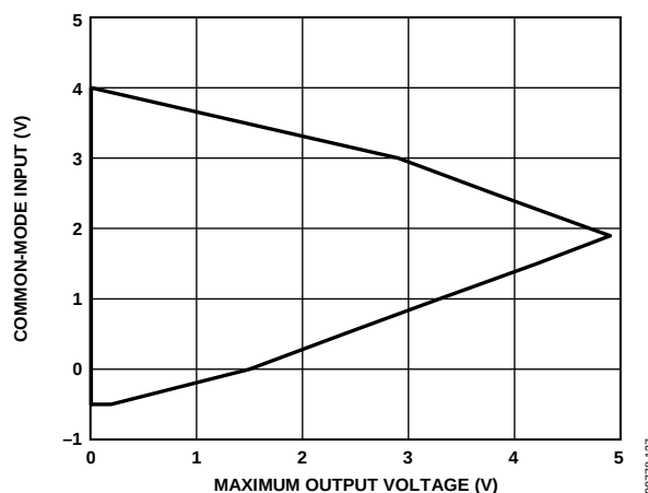
Figure 37. Common-Mode Input vs. Maximum Output Voltage, G \geq 10 , +V_S = 5 \text{ V} , -V_S = 0 \text{ V} , R_L = 100 \text{ k}\Omega , RM-8 and R-8 Package Options
