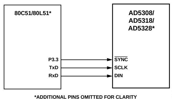
Figure 38. 80C51/80L51-to-AD5308/AD5318/AD5328 Interface
