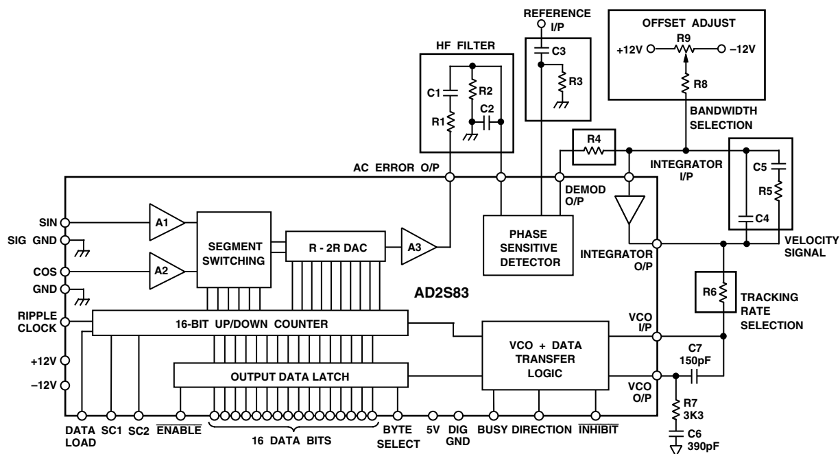
Figure 1. Connection Diagram
