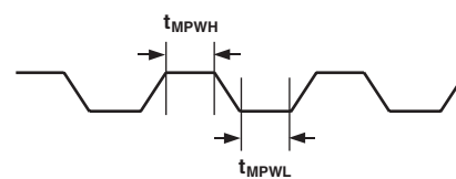
Figure 3. MCLK_IN Timing
