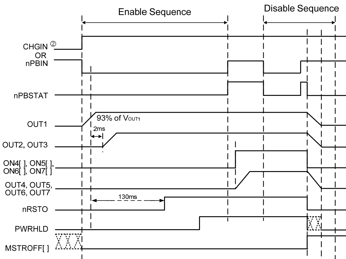
Enable/Disable Sequence
