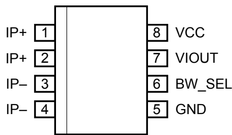
Pinout Diagram
