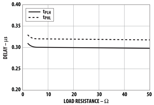
Figure 22. Propagation delay vs. load resistance.
