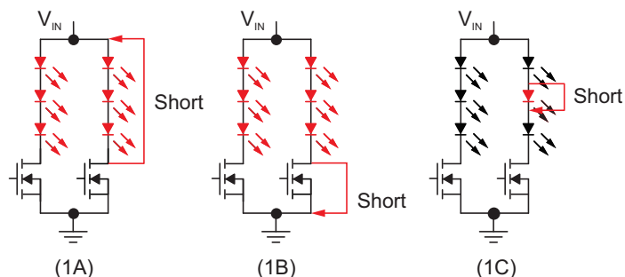
Figure 1: Short-Circuit Protection
