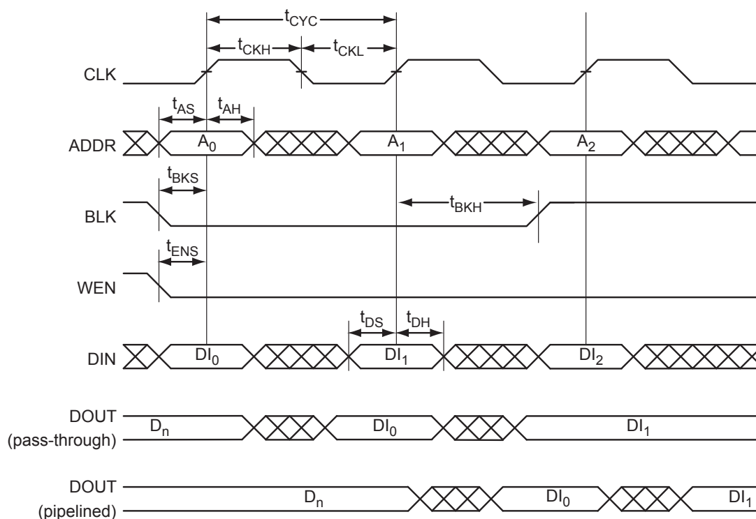
Figure 2-29 • RAM Write, Output as Write Data ( WMODE = 1 ). Applicable to both RAM4K9 only.
